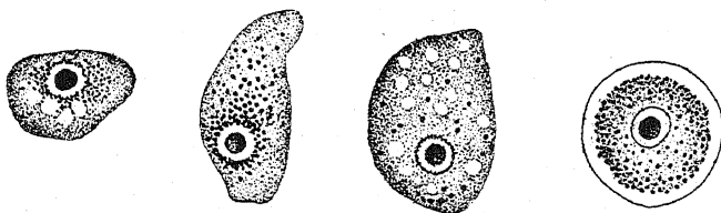
Ameba limax . Chromidia forming from nucleus and collecting in the cytoplasm prior to encystment.
